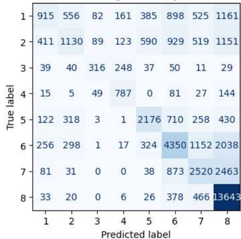
Confusion Matrix: Proving Ordinality via Clustered Errors
